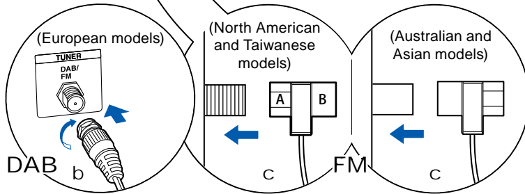
a AM loop antenna, b DAB/FM antenna, c Indoor FM antenna
